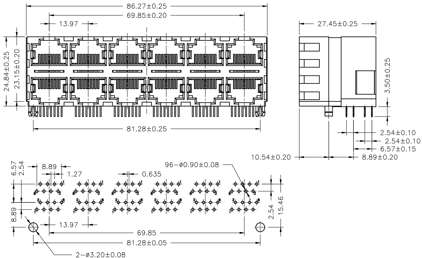
SUGGESTED PCB LAYOUT (COMPONENT SIDE)
