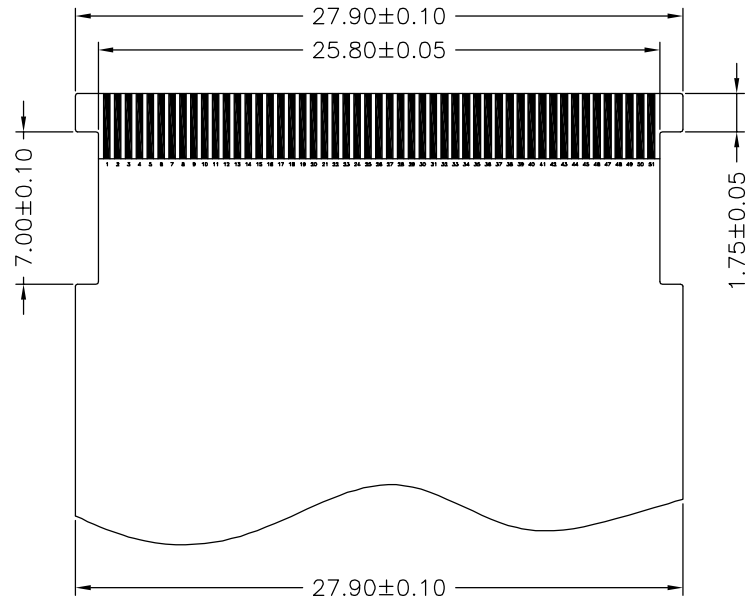
Recommended FFC dimension FFC T=0.40mm
