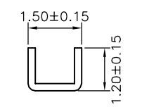
SEC:C-C
