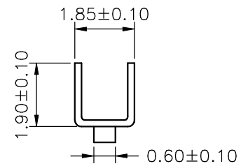
SEC:C-C
