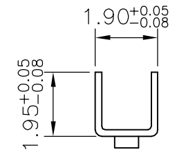
SEC:C-C
