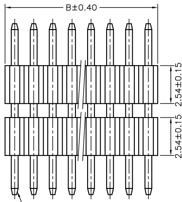
PIN 0.46 SQ
