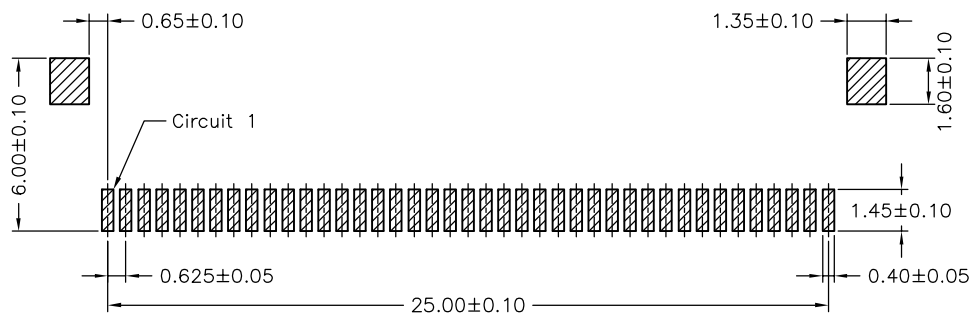
SUGGESTED PCB LAYOUT (COMPONENT SIDE)
